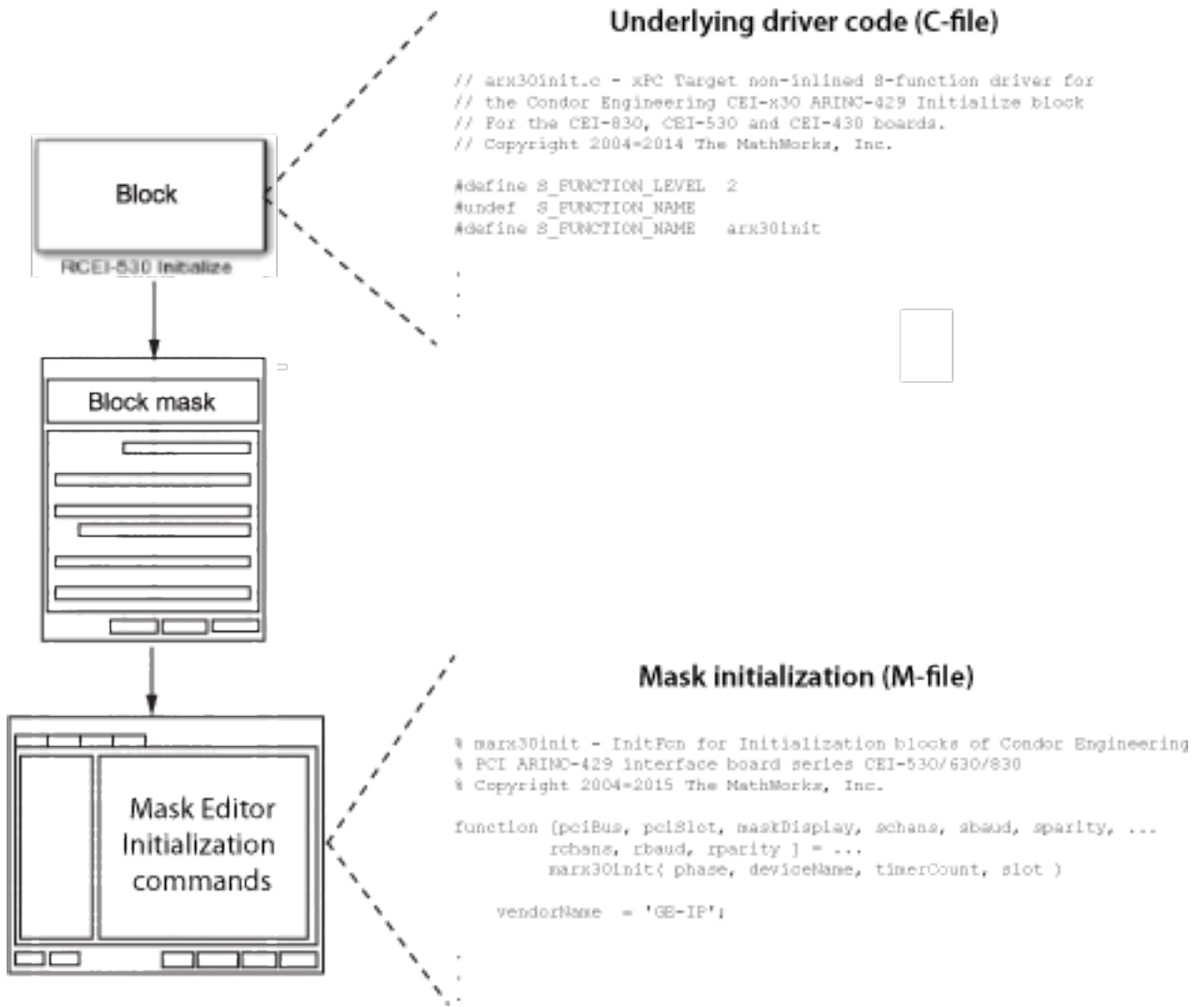
Anatomy of a Simulink Real-Time Driver
